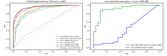
FIGURE 15. Anti-spoof ROC on CelebA-Spoof held-out ( n=600 ). The deployed depth-variance threshold (AUC 0.56) is barely above chance; the proposed 25-dim descriptor with an RBF-SVM reaches AUC 0.95, improving on reimplemented LBP+SVM (0.85) and HSV colour-texture (0.90) baselines with non-overlapping 95% CIs.
